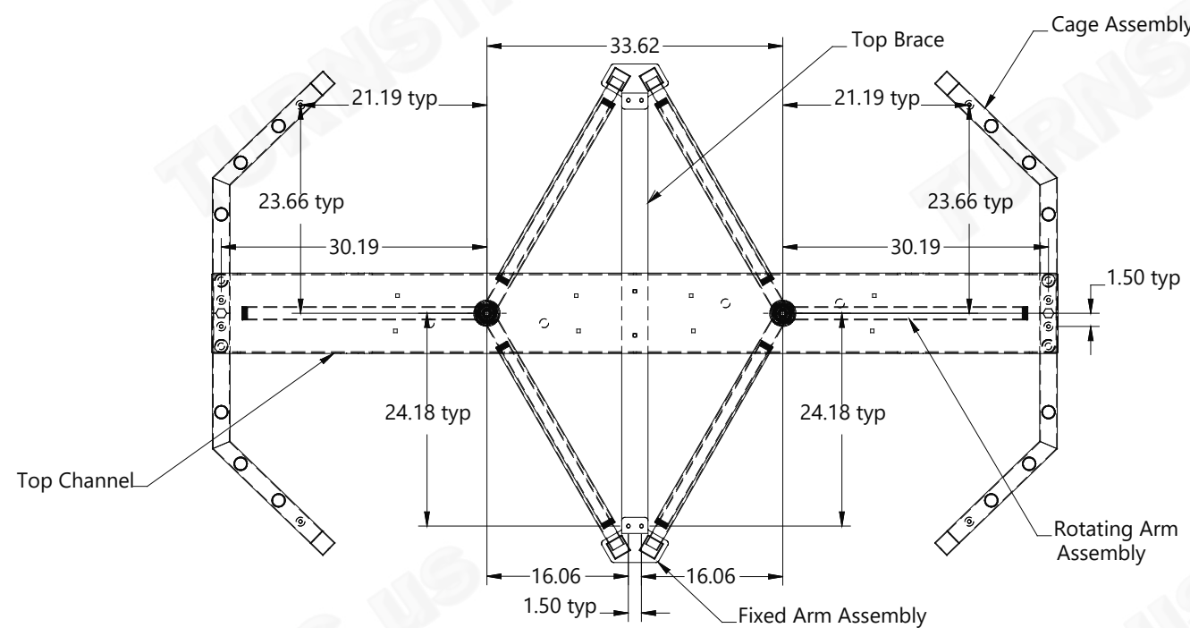
HT431T Mounting Hole Locations
