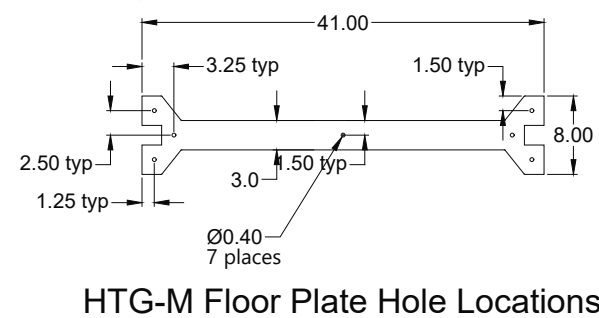
HTG-M Floor Plate Hole Locations
