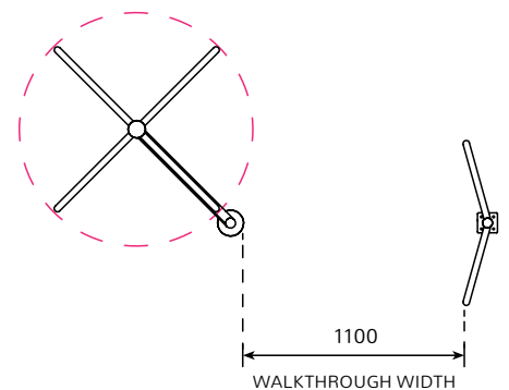
PLAN OPEN (SPECIAL NEEDS AREA)
