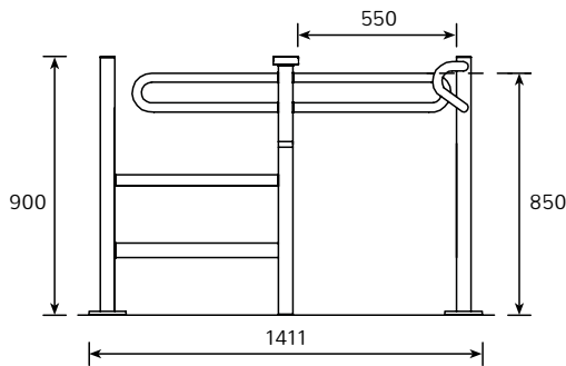
ENTRY / EXIT ELEVATION
