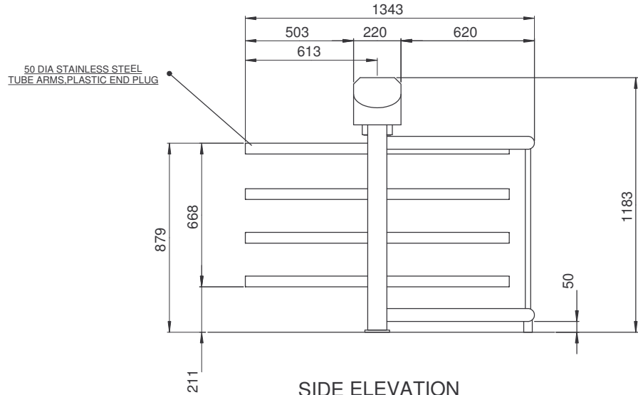
SIDE ELEVATION
