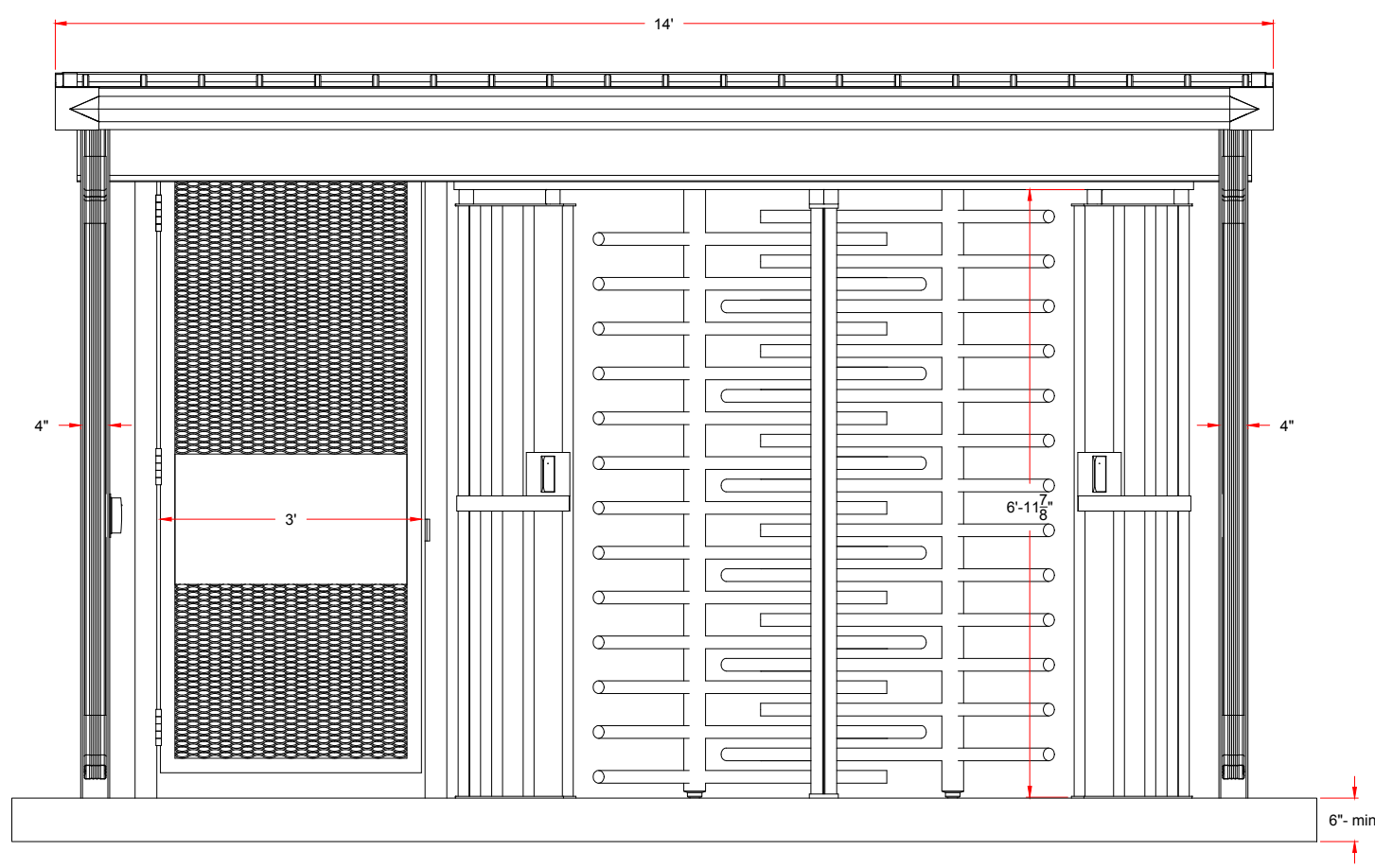
ELEVATION ENTRY SIDE
