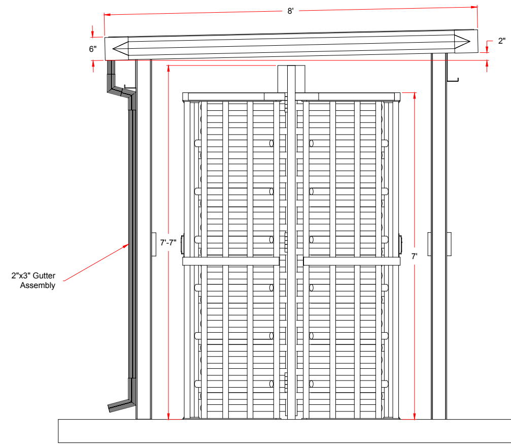
SIDE ELEVATION (heaters not shown)
