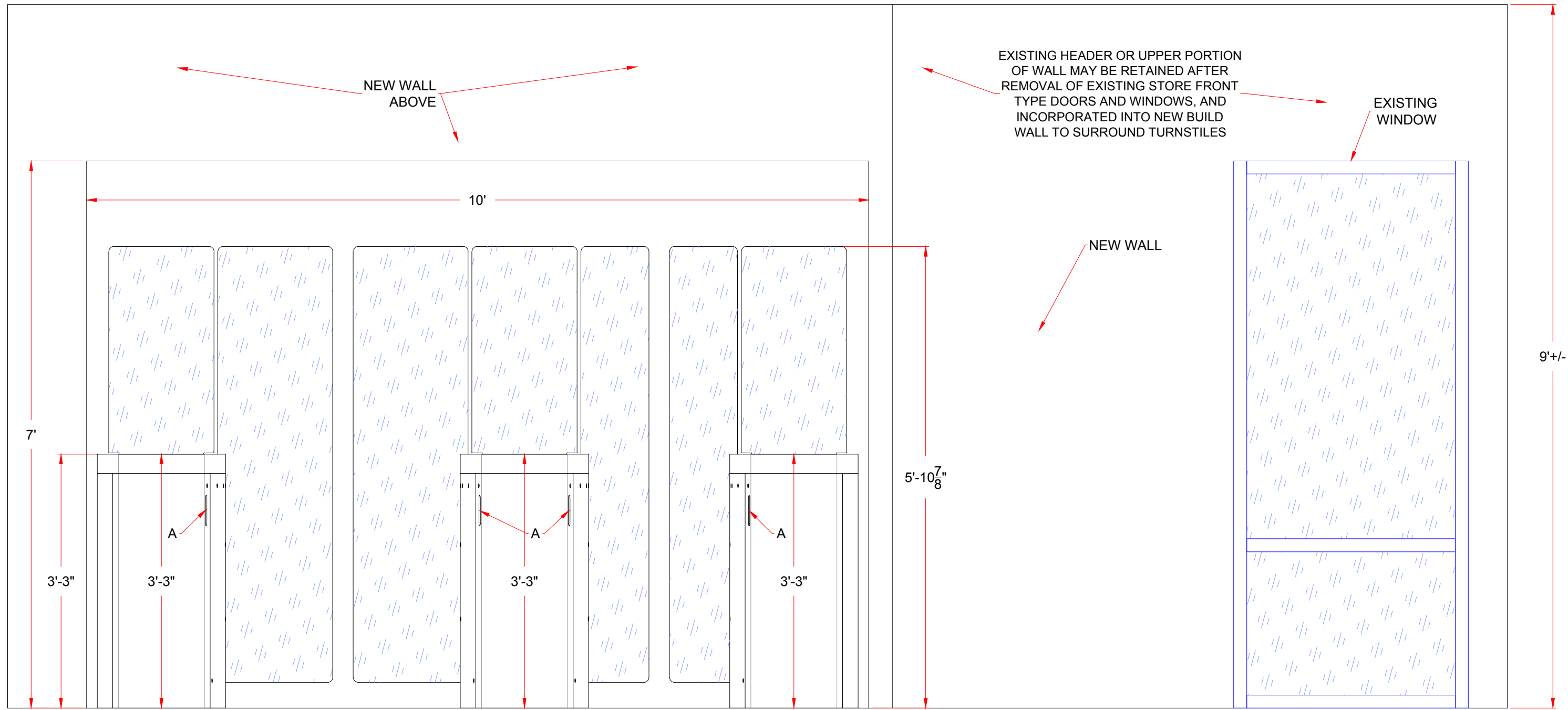
ELEVATION - ENTRANCE SIDE (exterior)
